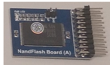
Fig. 1: A photo of the Waveshare NandFlash Board (A).
