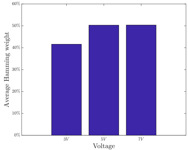
Fig. 4: Overall average fractional Hamming weight value of the examined NAND-Flash-memory-based PUF, for each value of supply voltage provided by the USB port of the STM32F429I-DISC1 board to the overall system.
