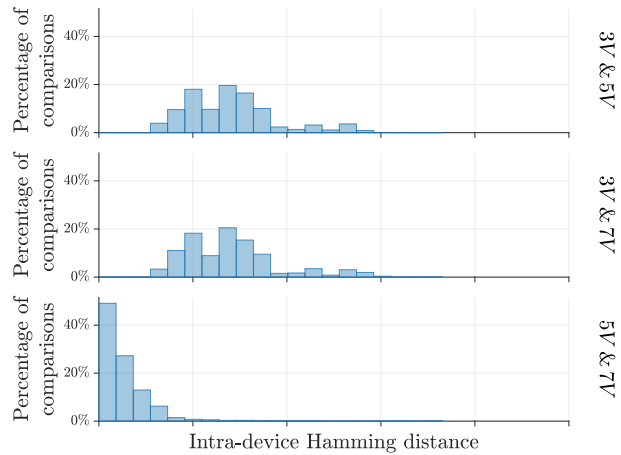
Fig. 5: Intra-device Hamming distance values for the examined NAND-Flash-memory-based PUF, for pairs of PUF responses taken at different supply voltage levels provided by the USB port of the STM32F429I-DISC1 board to the overall system.
